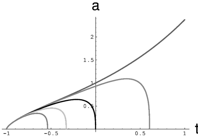
FIG. 4. Expansion of the universe for \Lambda = 0.7\rho_0 . The upper line corresponds to the fiducial model with \phi_0 = 0 (cosmological constant; field does not move). The line below corresponds to \phi = 0.5 . The next line corresponds to \phi = 1 , then to \phi = 1.5 , and \phi = 2 .
