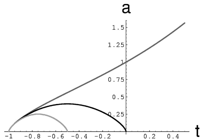
FIG. 1. Evolution of a flat \Lambda CDM universe for various values of \Lambda . Time is in units of the present age of the universe t_0 \approx 14 \times 10^9 years. The present moment is placed at t=0 , the big bang corresponds to t=-1 . The upper line corresponds to the flat universe with \Omega_{\text{tot}}=1 , \Omega_\Lambda=0.7 (i.e. \Lambda=+0.7\rho_0 ) and \Omega_M=0.3 . The next line below it corresponds to a flat universe with \Lambda=-4.7\rho_0 . As we see, this universe collapses at the age of 14 \times 10^9 years. The total lifetime of the universe with \Lambda=-18.8\rho_0 (the lower line) is only 7 \times 10^9 years.
